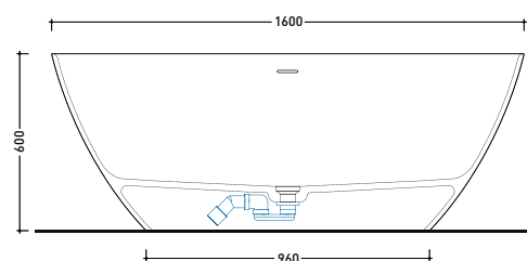
vista frontale / frontal view
